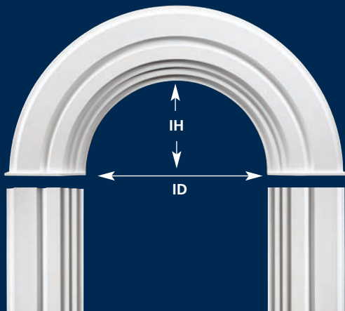
10 1/8" Window Arch
