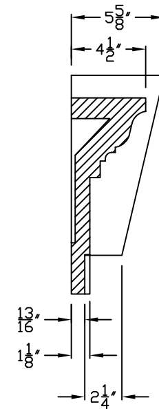
SEC :A-A
